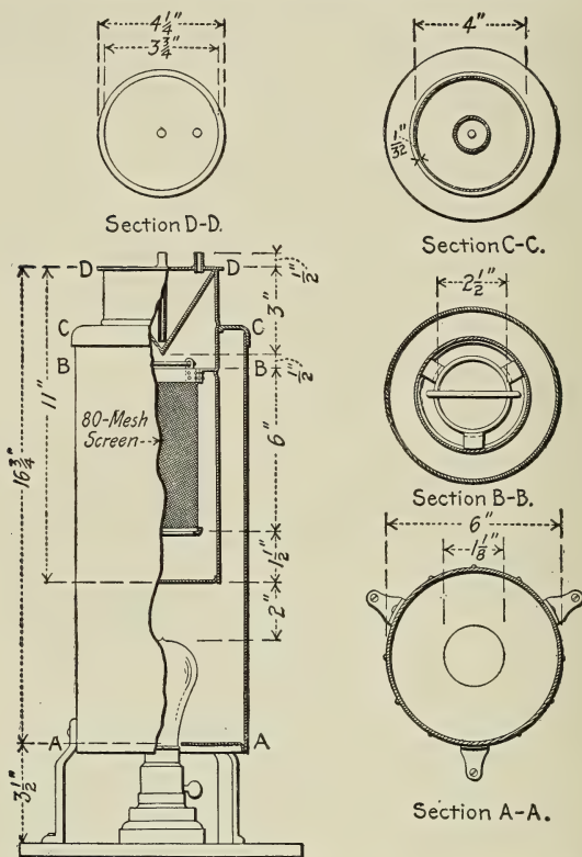
FIG. 196.—Forrest's Hot-extraction Apparatus.
